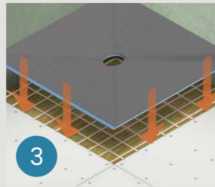
3 Installing base
